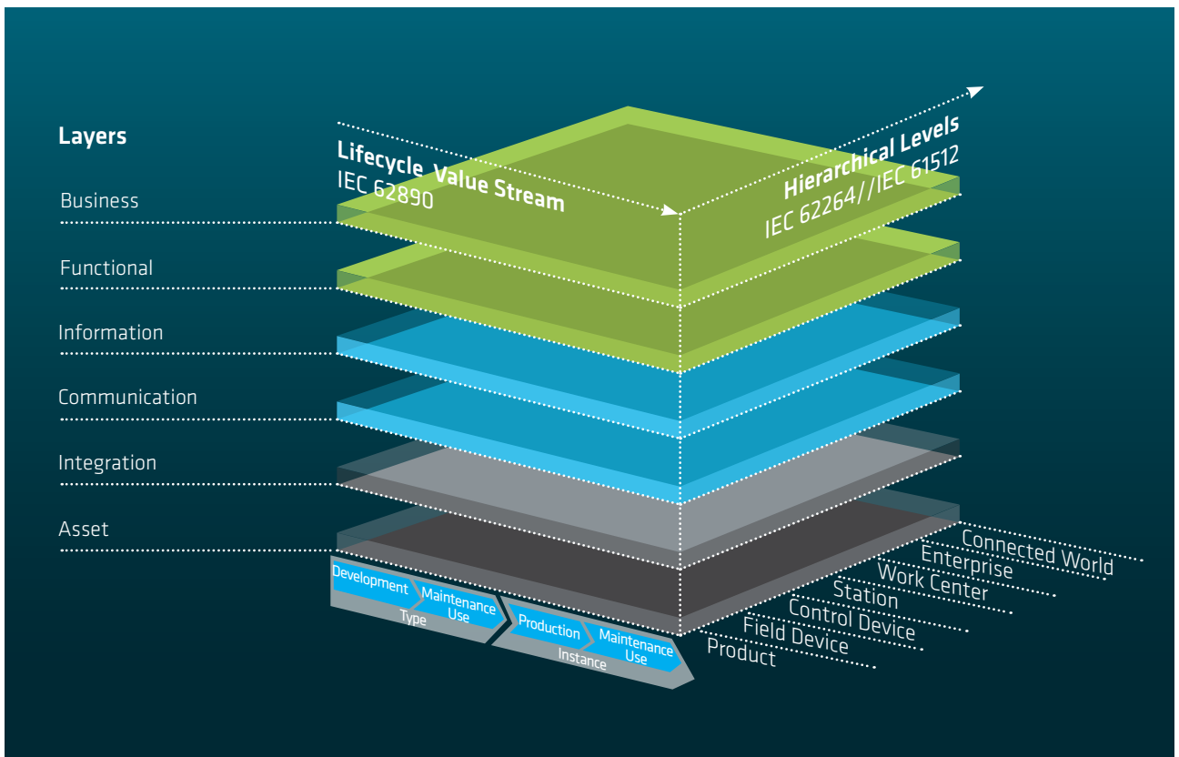
Fig. 1: RAMI 4.0 model
