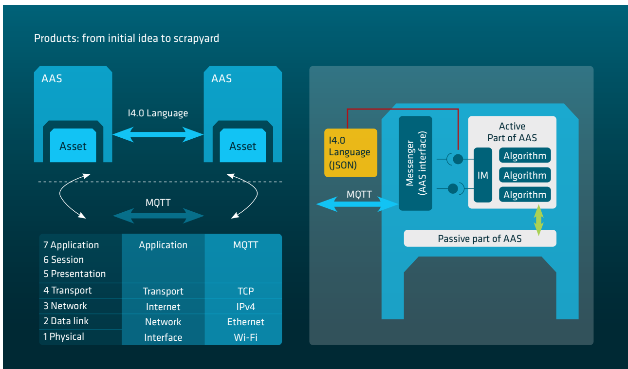
Fig. 9: Active AAS and use of I4.0 language in the ISO/OSI model [15]
