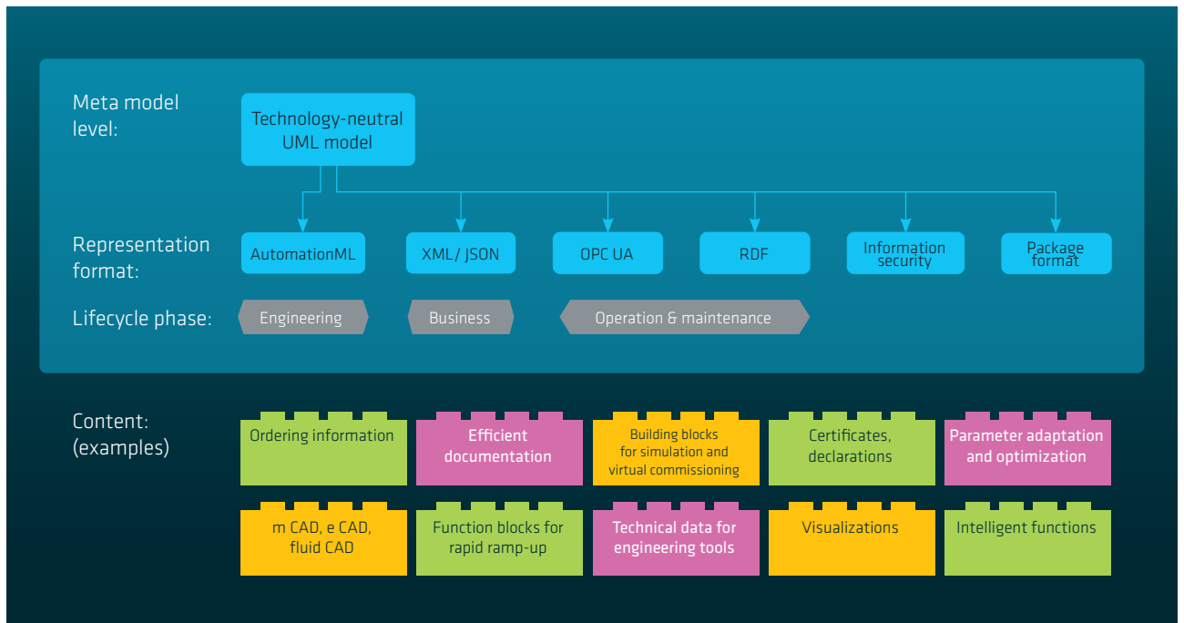
Fig. 3: AAS over its lifecycle [21]
