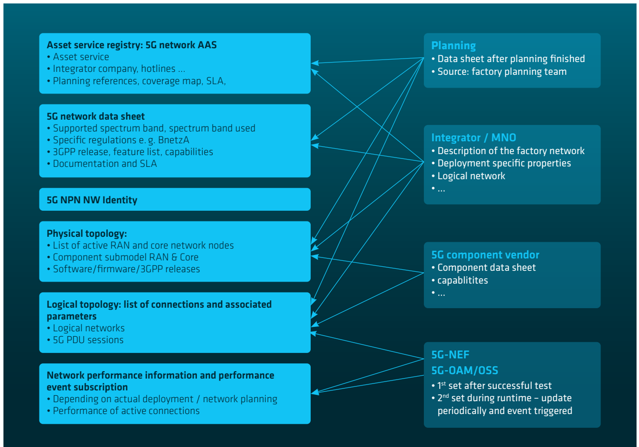
Fig. 21: Example of a hierarchical 5G AAS and information sources during its lifecycle
