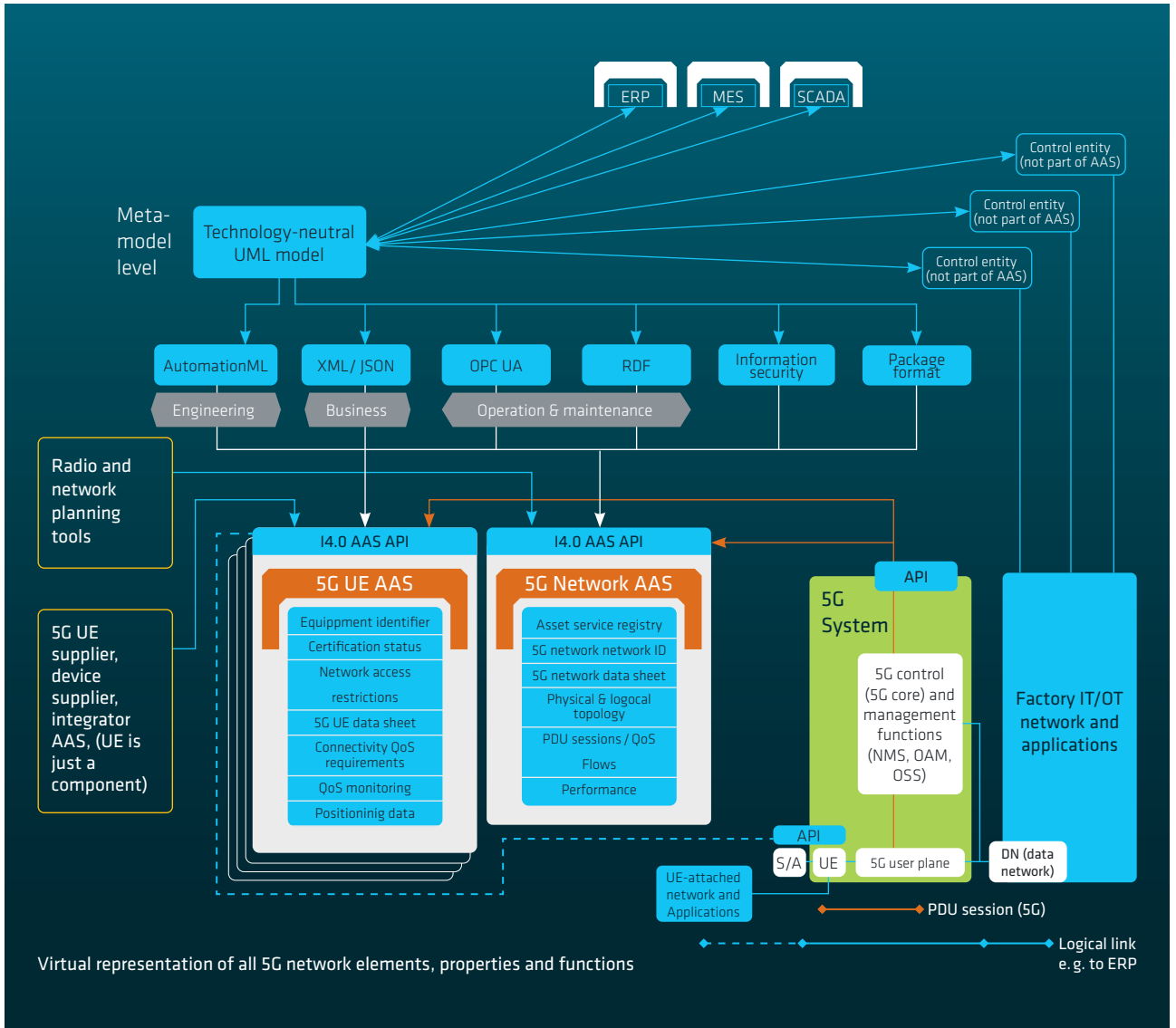
Fig. 20: Virtual representation of all 5G network components, functions, and KPIs in AAS
