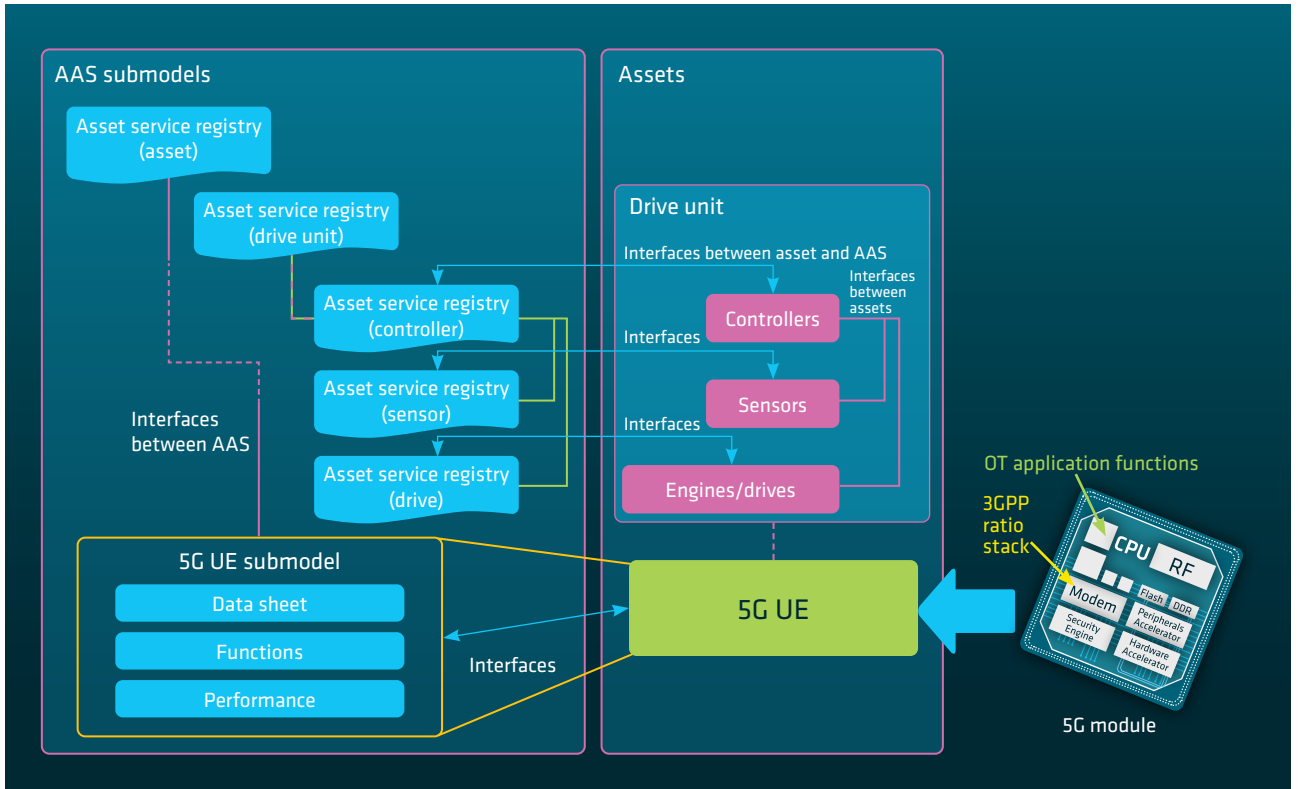
Fig. 17: Illustration of the relationship between a physical world asset and 5G UE
