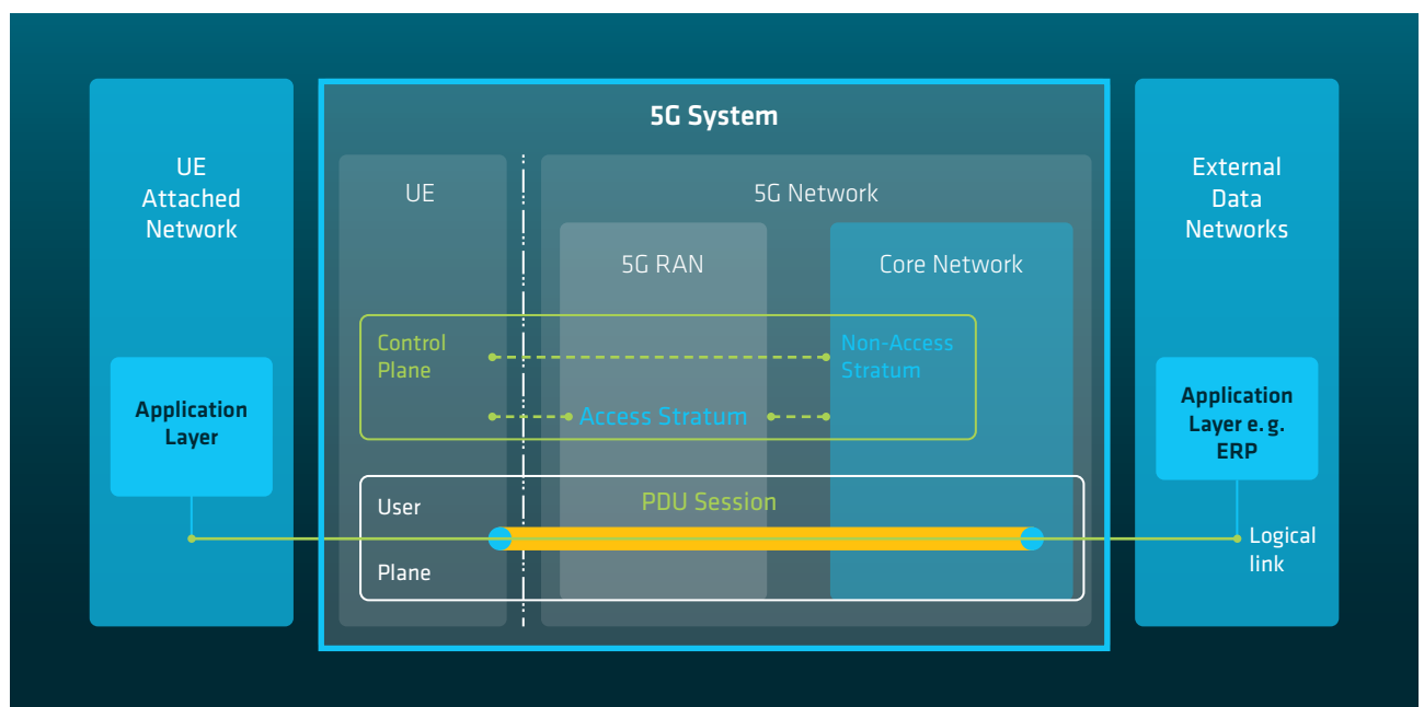
Fig. 10: 5G system functional domains and planes
