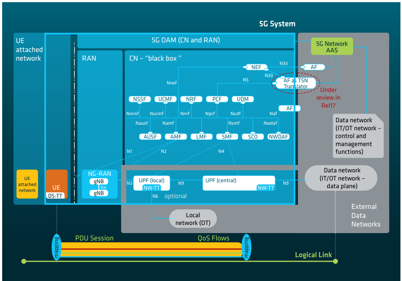
Fig. 11: 5G architecture with service-based CN architecture representation
