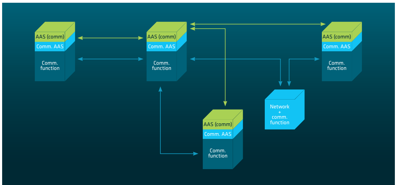
Fig. 4: An automation network described in an AAS "communication" layer [28]
