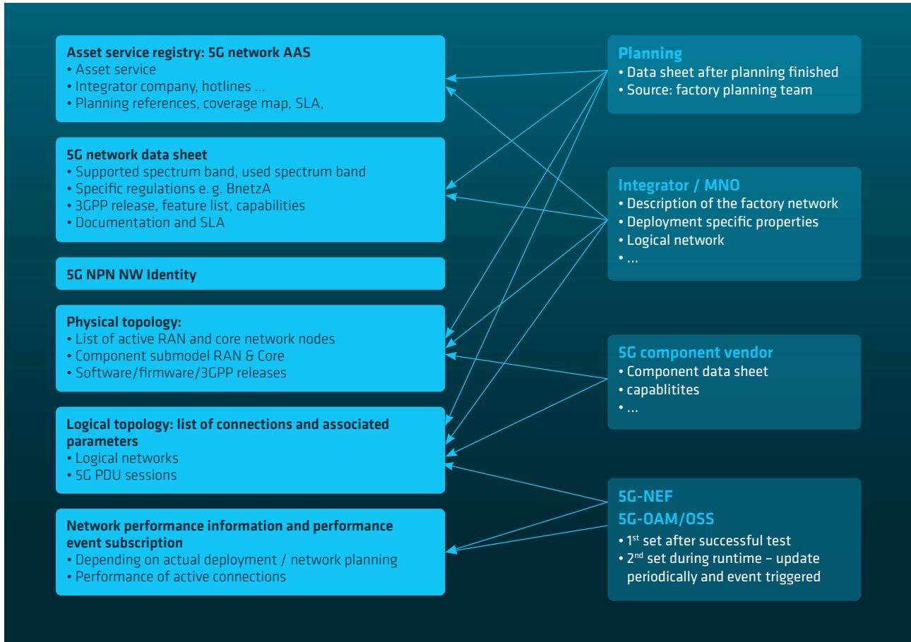
Fig. 16: Stakeholders accessing 5G network AAS
