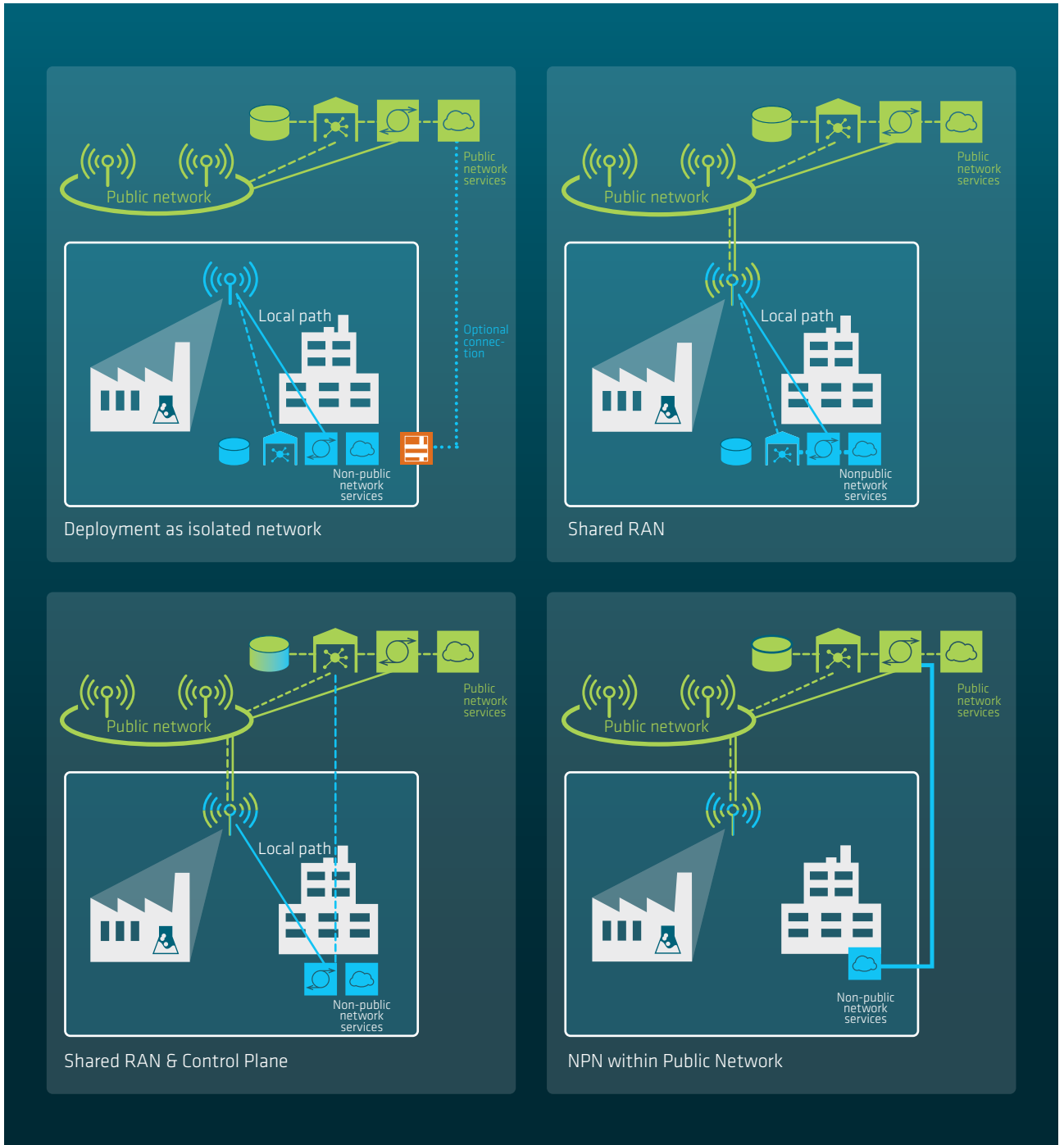
Fig. 14: Four examples of NPN deployments in conjunction with public networks [3]
