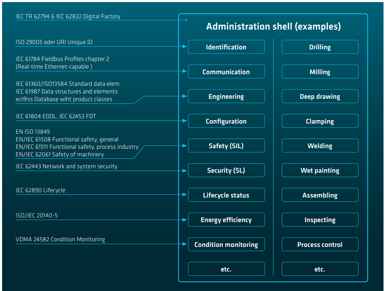
Fig. 5: Possible submodels of an AAS [16][23]
