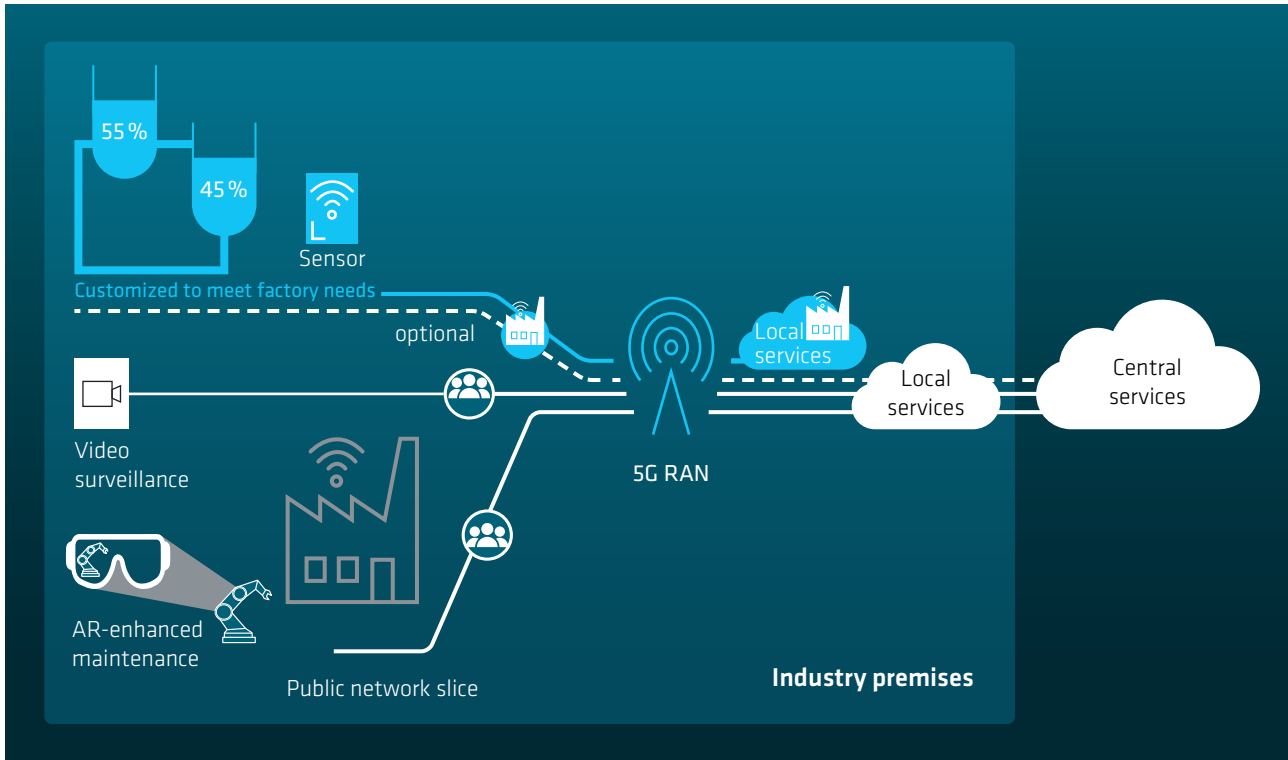
Fig. 12: Network slicing at an industrial facility
