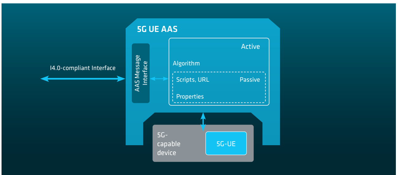
Fig. 18: Internal structure of the 5G UE AAS
