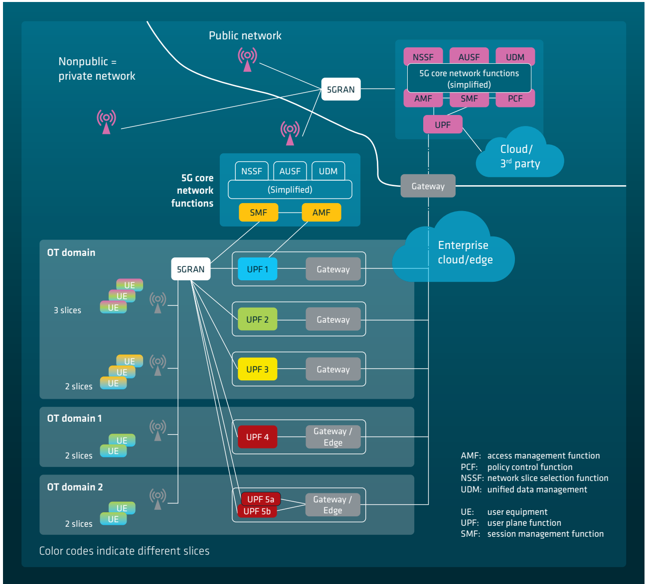
Fig. 22: Flexible cross-layer communication by multiple slices
