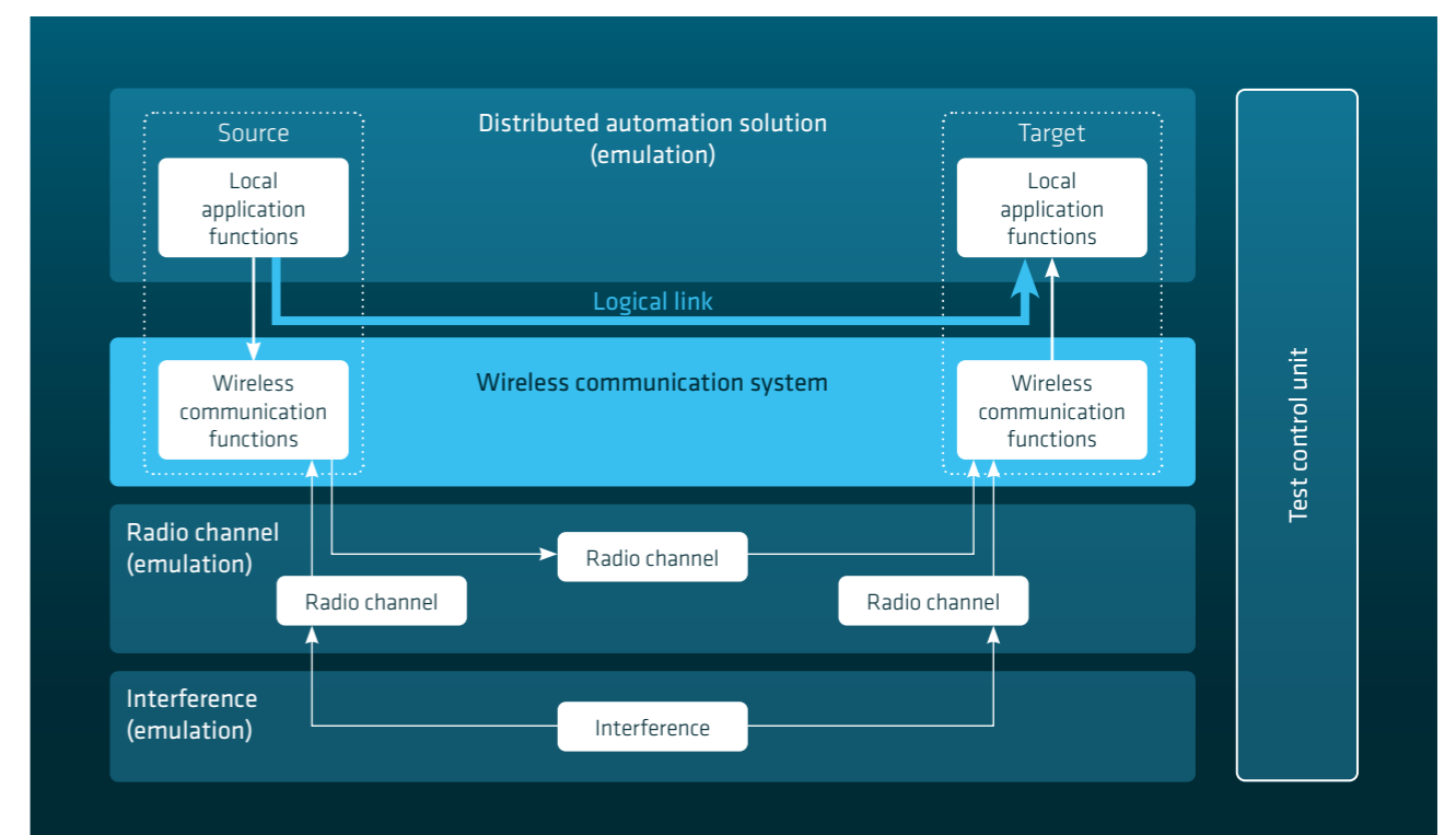
Fig. 10: SUT: Logical link
