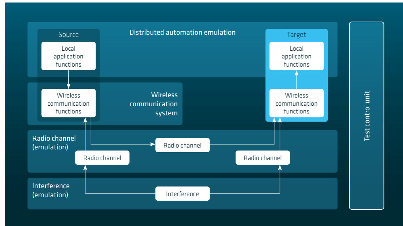
Fig. 8: SUT: Wireless device or communication module
