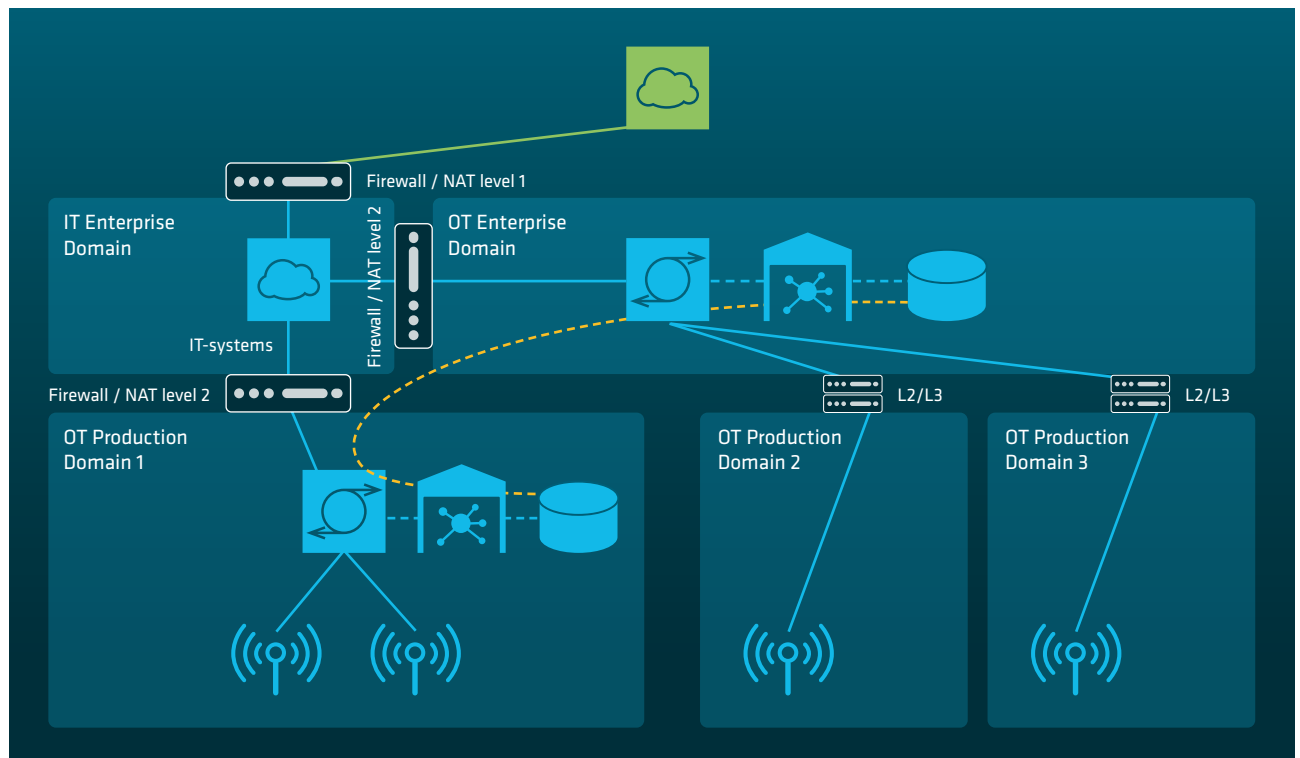
Figure 8: Private 5G NPN deployment: manufacturing enterprise
