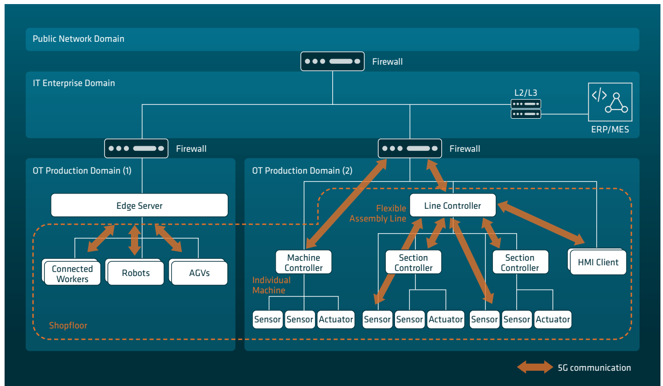
Figure 2: Logical view of an industrial network for a manufacturing building
