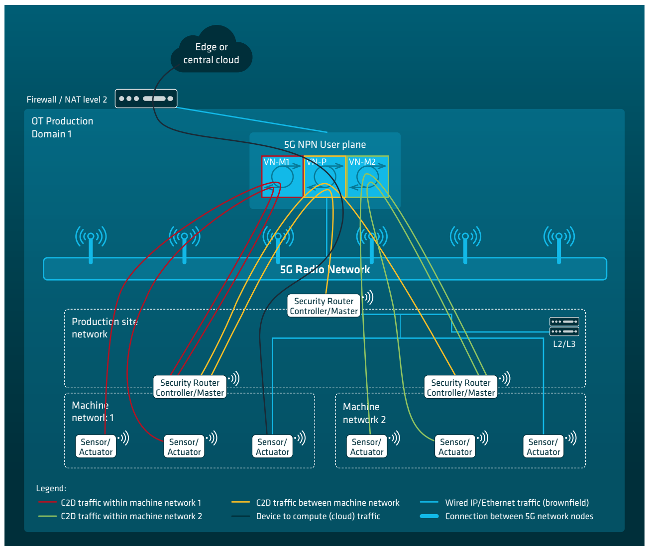
Figure 10: User plane data streams for dedicated NPN installation: manufacturing enterprise
