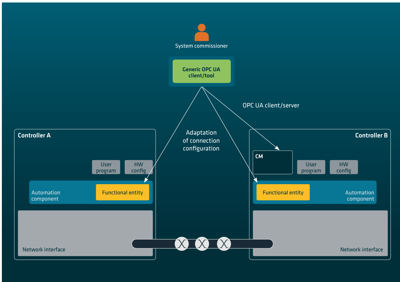
Figure 8: Connection commissioning
