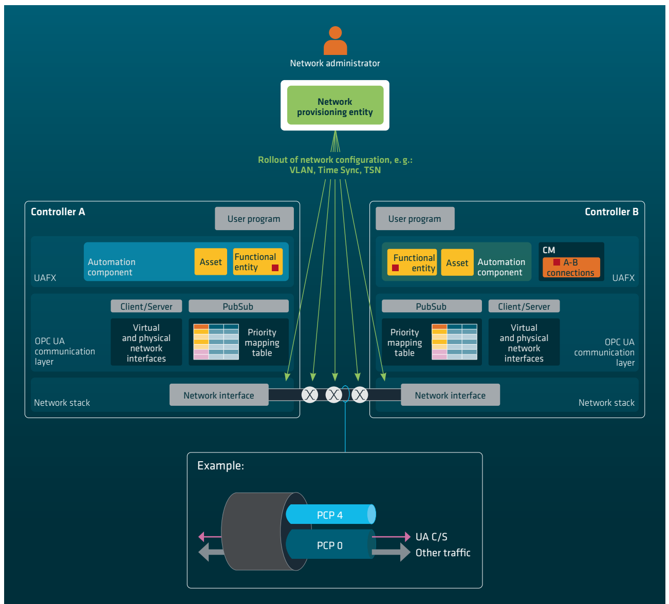
Figure 7: Network configuration
