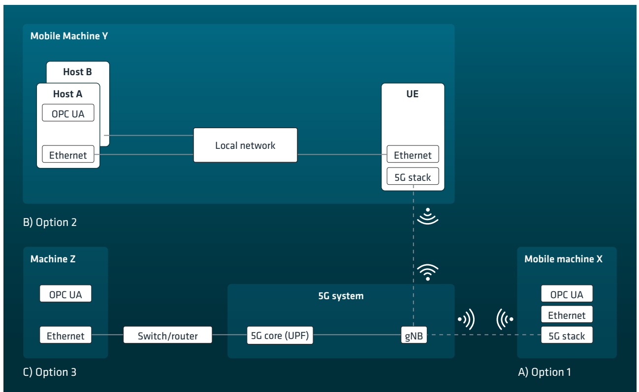
Figure 11: Ethernet-based OPC UA application deployment options
