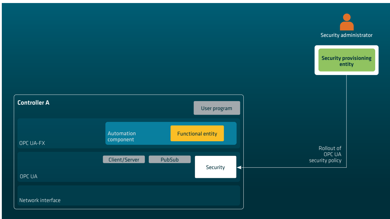
Figure 6: Security configuration
