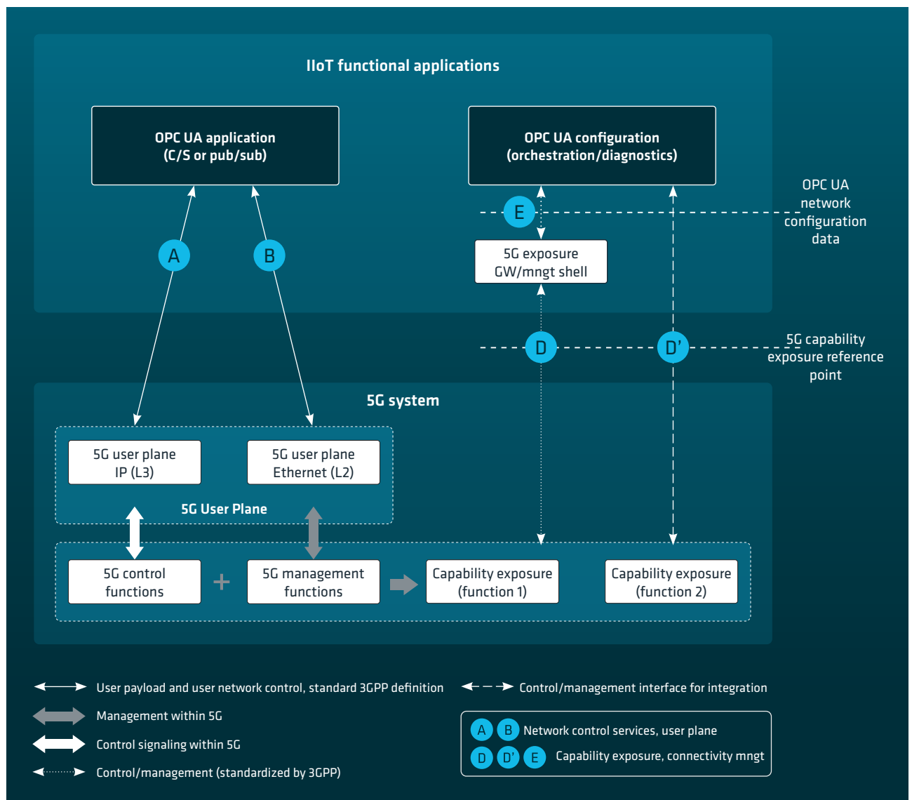
Figure 12: High-level system architecture for integrating OPC UA and 5G
