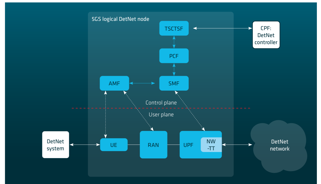
Figure 10: Architecture for 5GS interworking with DetNet
